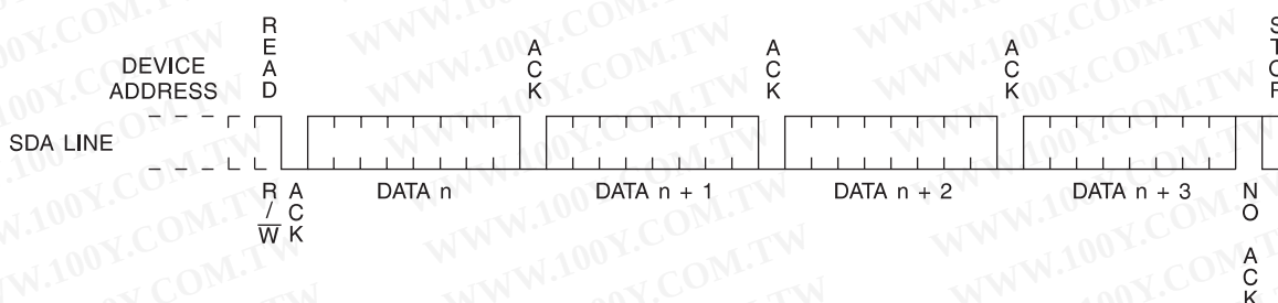
Figure 6. Sequential Read
