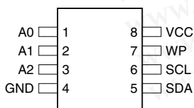
8-lead PDIP
