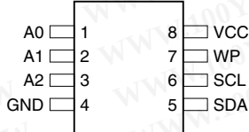
8-lead SOIC
