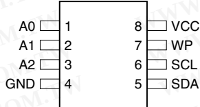
8-lead TSSOP
