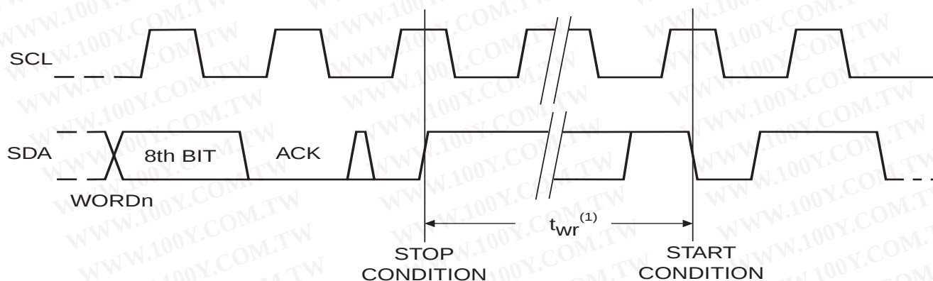
Figure 4. SCL: Serial Clock, SDA: Serial Data I/O
