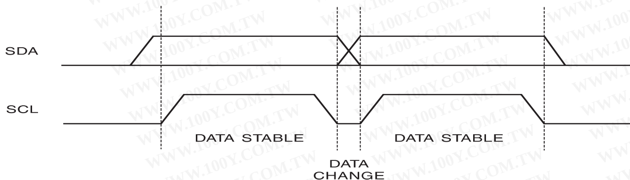
Figure 5. Data Validity
