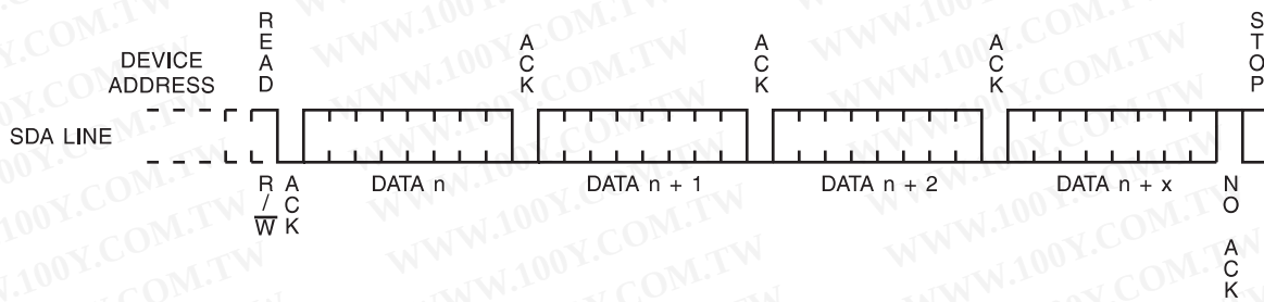
Figure 13. Sequential Read
