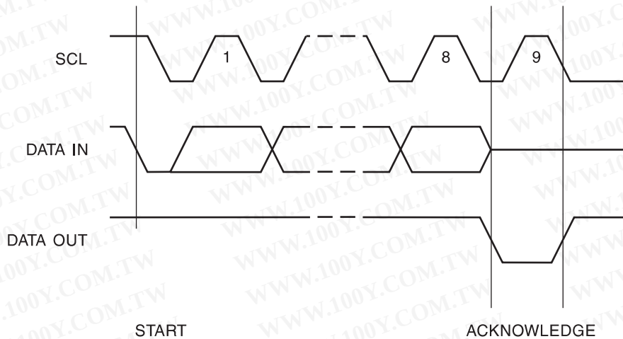
Figure 7. Output Acknowledge
