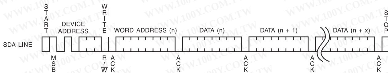
Figure 10. Page Write
