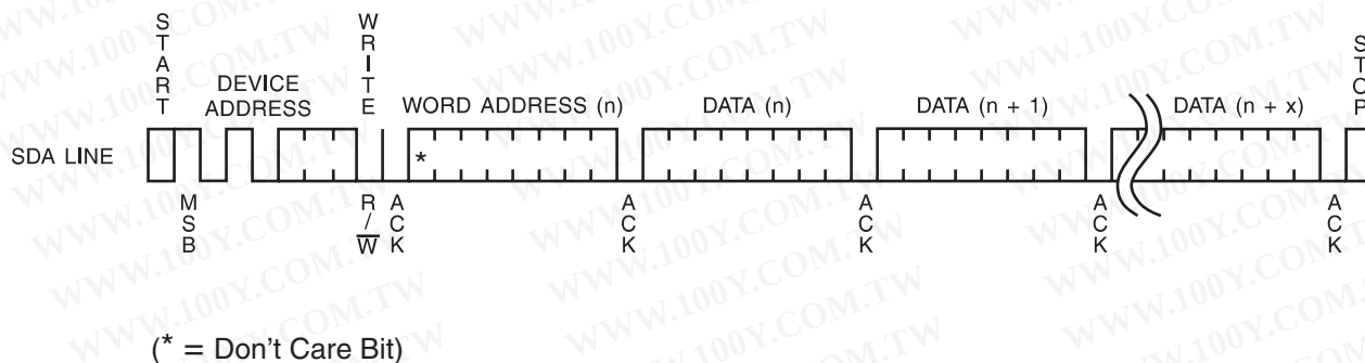
Figure 9. Page Write
