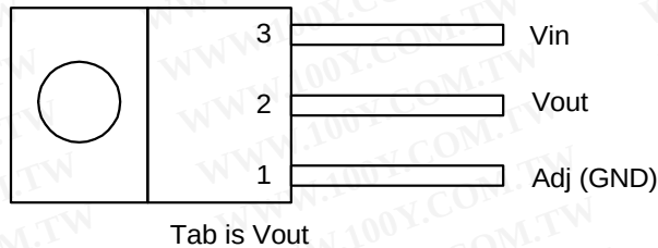
3 PIN TO220
