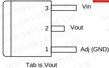
3 PIN TO220
