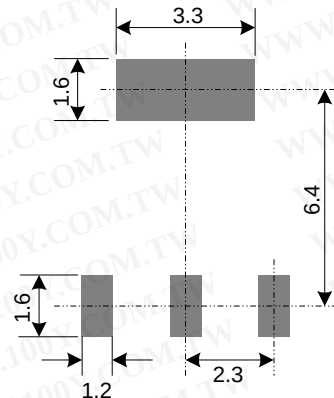
Land Pattern Recommendation (Unit: mm)
