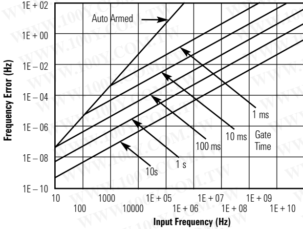
Graph 4: Agilent 53132A—Worst Case RMS Resolution? (Automatic or External Arming)
