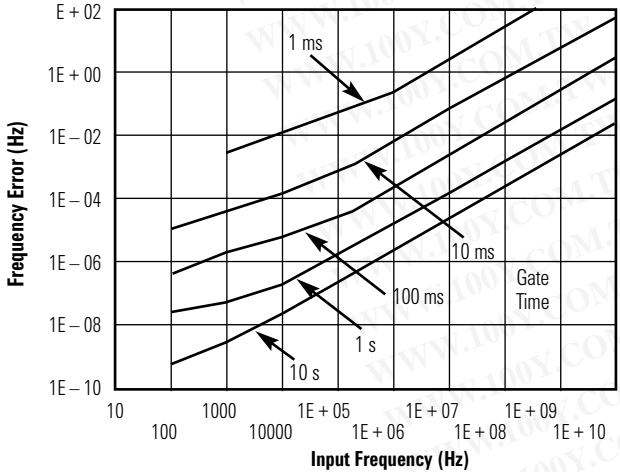
Graph 5: Agilent 53132A—Worst Case RMS Resolution? (Time or Digits Arming)
