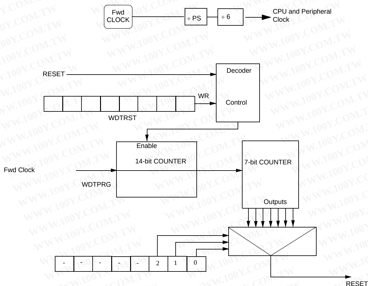
Figure 38. Watchdog Timer
