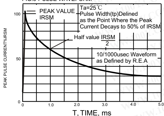
FIG.5-PULSE WAVEFORM
