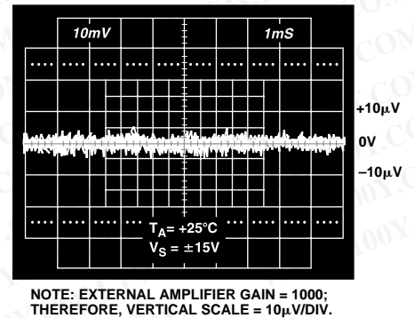
Figure 18. Voltage Noise from 0 kHz to 1 kHz
