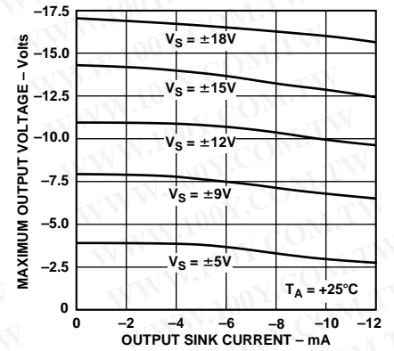
Figure 15. Maximum Output Voltage vs. Output Current (Sink)
