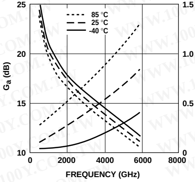
Figure 14. Fmin and G_a vs. Frequency and Temperature at V_{DS} = 4 V, I_{DS} = 60 mA.
