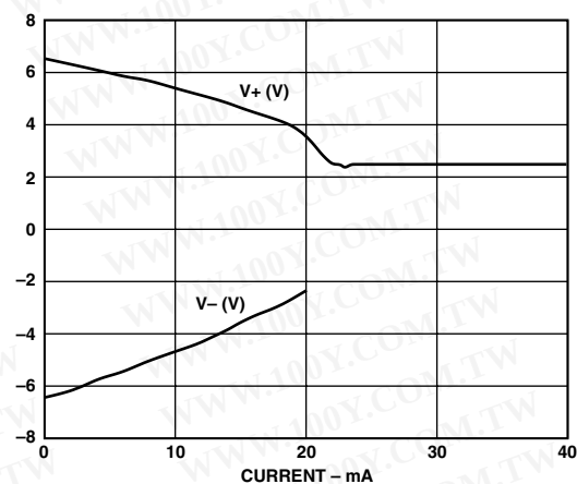
Figure 4. Charge Pump V+, V- vs. Current
