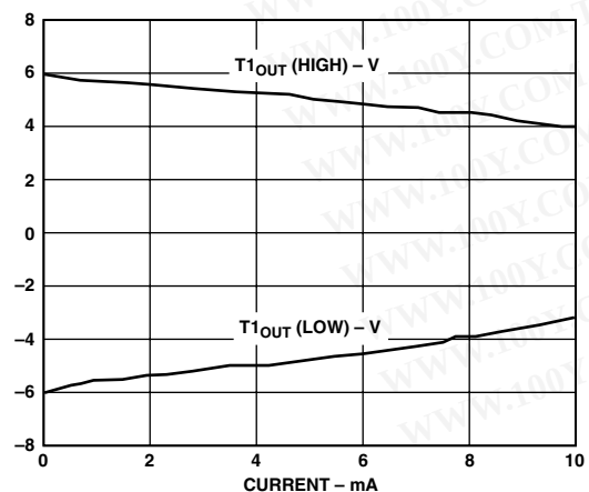
Figure 3. Transmitter Output Voltage Low/High vs. Load Current
