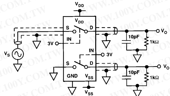
TEST CIRCUIT 6 CHANNEL-TO-CHANNEL CROSSTALK
