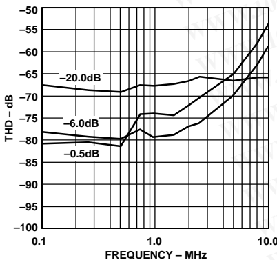
Figure 17. THD vs. Input Frequency (Input Span = 5.0 V p-p, V_{\text{CM}} = 2.5 \text{ V} )
