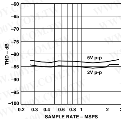
Figure 9. THD vs. Sample Rate (A IN = -0.5 dB, f IN = 500 kHz, V CM = 2.5 V)
