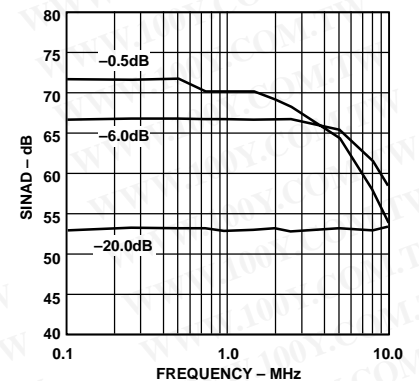
Figure 16. SINAD vs. Input Frequency (Input Span = 5.0 V p-p, V_{\text{CM}} = 2.5 \text{ V} )
