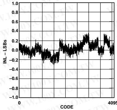
Figure 3. Typical INL
