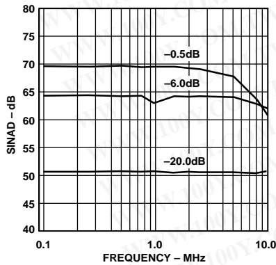
Figure 14. SINAD vs. Input Frequency (Input Span = 2.0 V p-p, V_{\text{CM}} = 2.5 \text{ V} )
