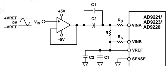
Figure 41. AC-Coupled Input
