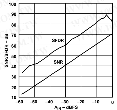
Figure 19. SNR/SFDR vs. A_{\text{IN}} (Input Amplitude) ( f_{\text{IN}} = 1.5 \text{ MHz} , Input Span = 2 V p-p, V_{\text{CM}} = 2.5 \text{ V} )
