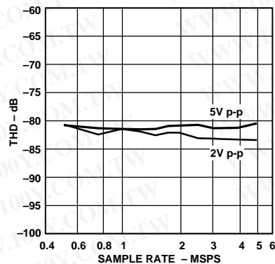
Figure 18. THD vs. Sample Rate ( A_{\text{IN}} = -0.5 \text{ dB} , f_{\text{IN}} = 500 \text{ kHz} , V_{\text{CM}} = 2.5 \text{ V} )
