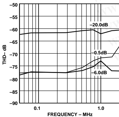
Figure 8. THD vs. Input Frequency (Input Span = 5.0 V p-p, V CM = 2.5 V)
