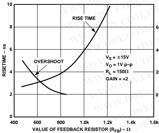
Figure 9. Rise Time and Overshoot vs. Value of Feedback Resistor, R_{FB}
