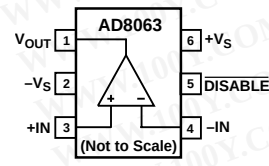
Figure 3. 6-Lead SOT-23 (RT)
