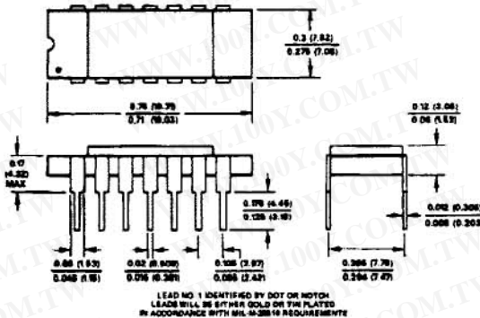
AD7592DI
