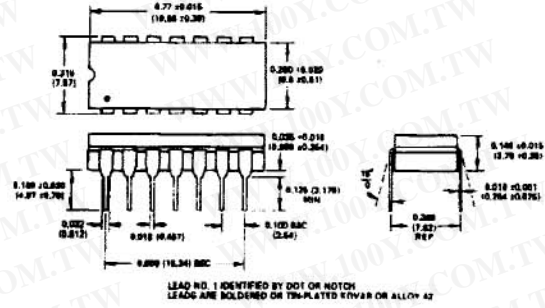
AD7592DI
