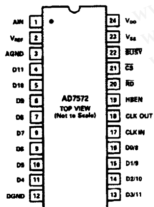
DIP
