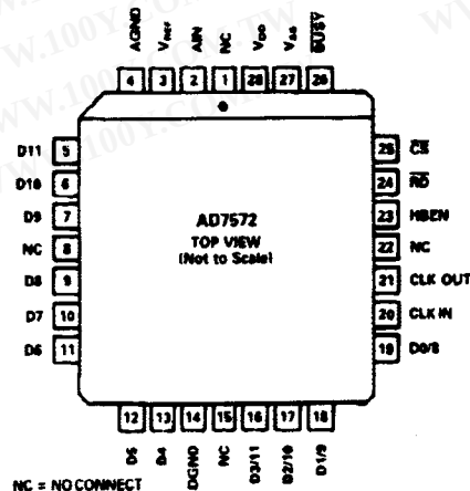
PLCC
