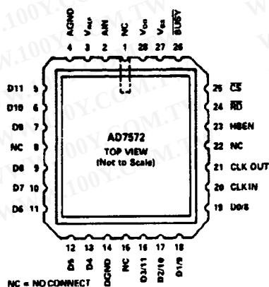
LCCC
