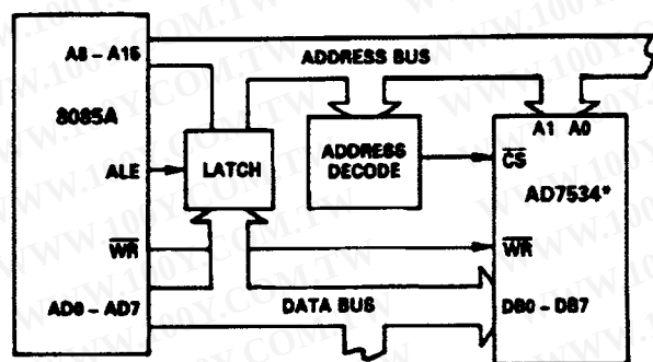
Figure 9. AD7534 - 8085A Interface
