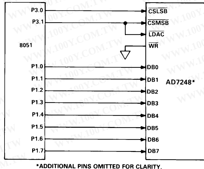
Figure 18. AD7248 to MCS-51 Interface
