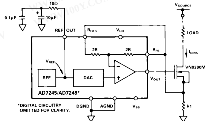
Figure 10. Programmable Current Sink
