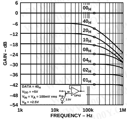
Figure 16. 50 kΩ Gain vs. Frequency vs. Code
