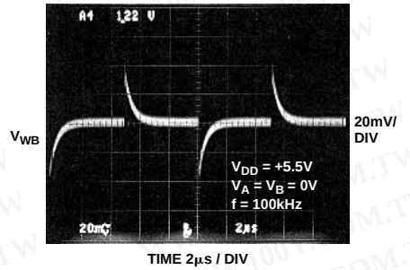
Figure 18. Digital Feedthrough
