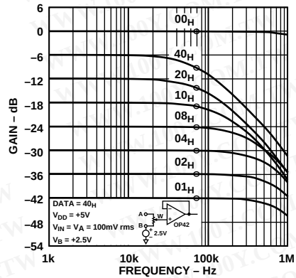
Figure 17. 100 kΩ Gain vs. Frequency vs. Code
