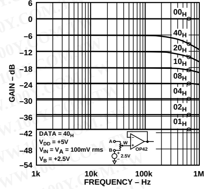
Figure 15. 10 kΩ Gain vs. Frequency vs. Code
