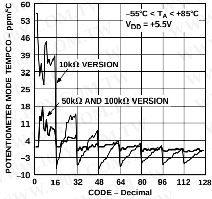
Figure 13. \Delta V_{WB}/\Delta T Potentiometer Mode Tempco (10 kΩ and 50 kΩ)
