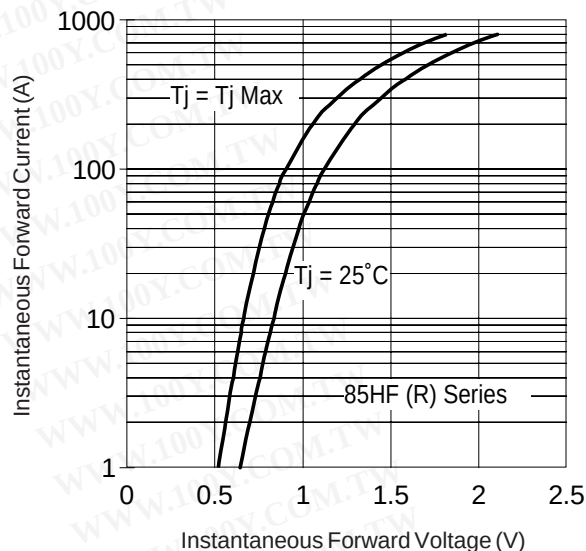
Fig. 12 - Forward Voltage Drop Characteristics (for 1400V, 1600V)
