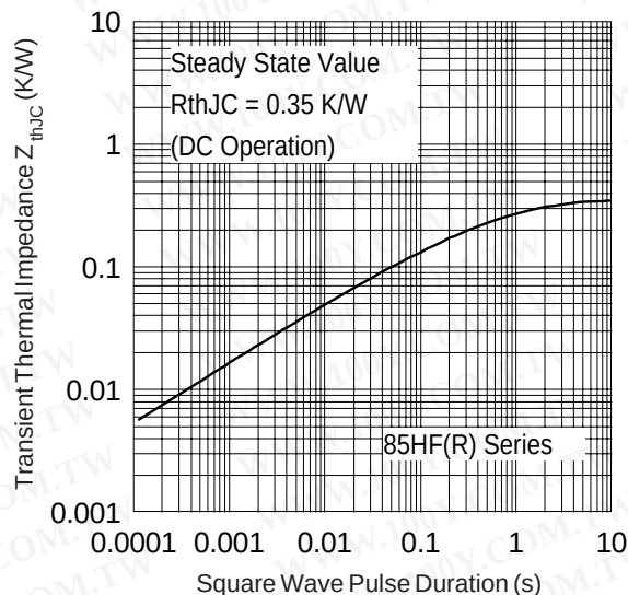
Fig. 13 - Thermal Impedance Z_{thJC} Characteristics
