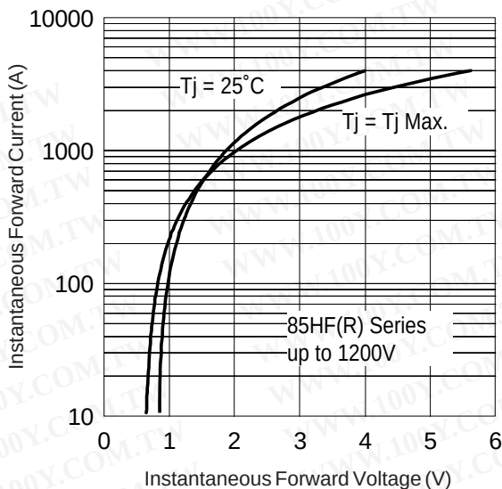
Fig. 11 - Forward Voltage Drop Characteristics (up to 1200V)
