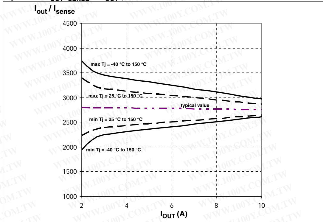
Figure 8. Maximum current sense ratio drift vs load current (a)
