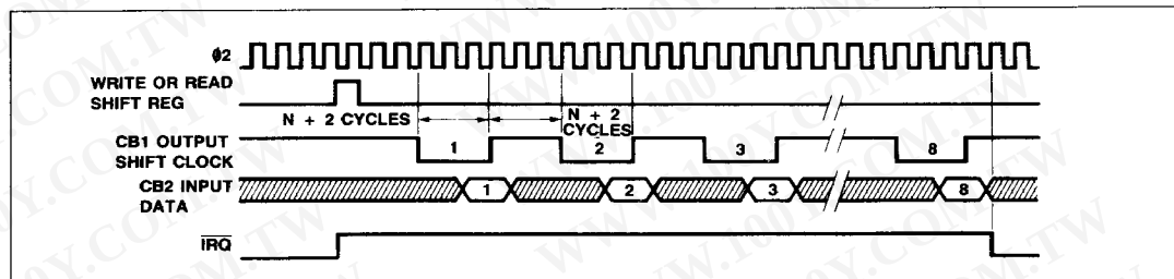
Figure 20. Shift Register
