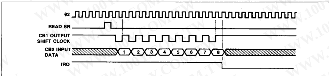
Figure 23. SR Mode 2 — Shift In Under Ø2 Control
