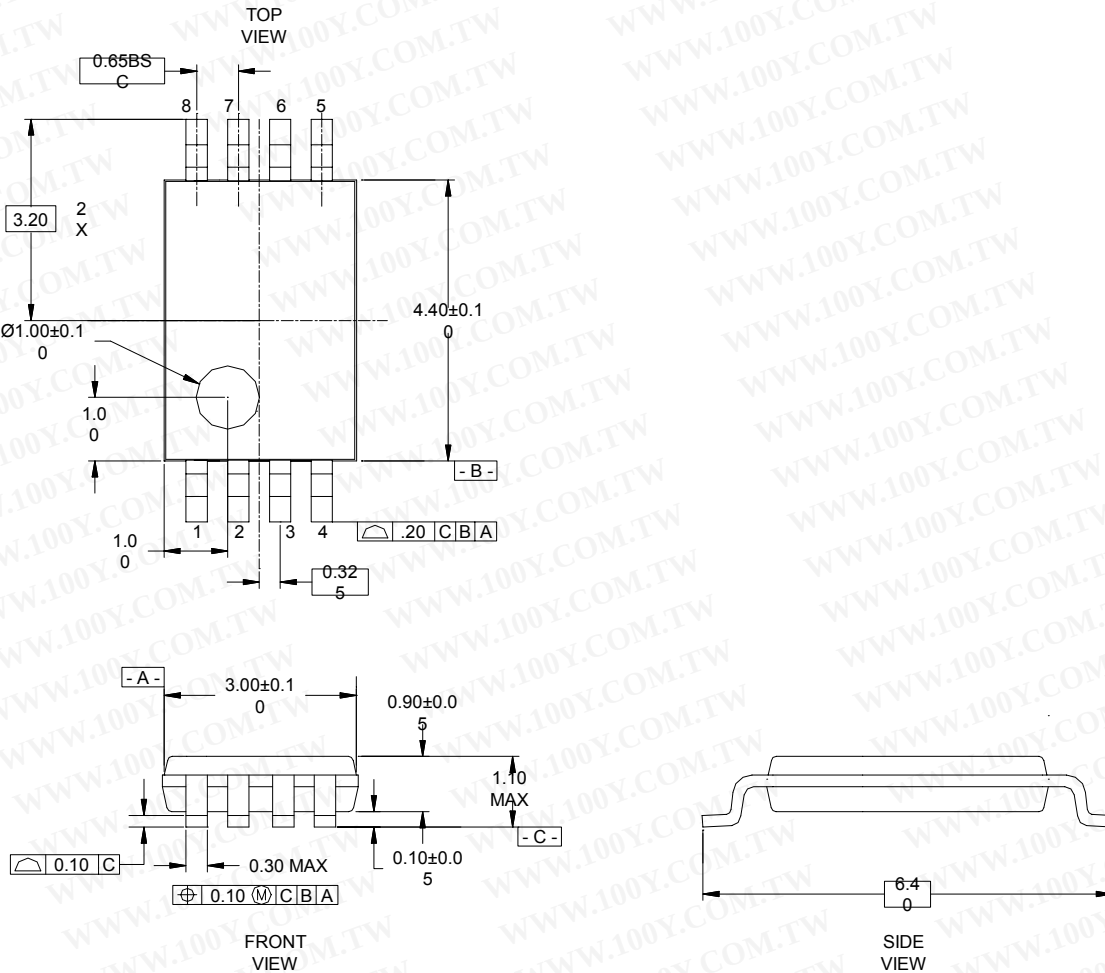
Figure 12. Package Drawing
