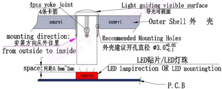
安装示意装配图 Installation schematic assembly drawing
