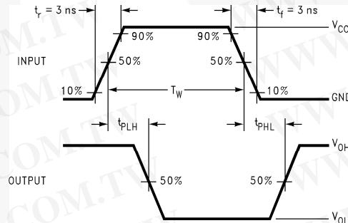
Figure 5. AC Waveforms
