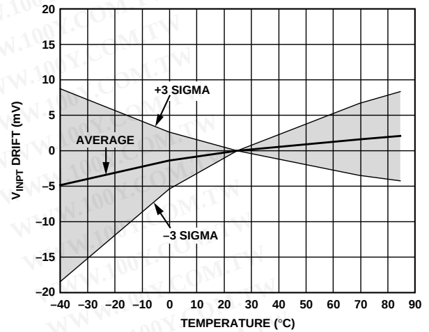
Figure 12. Temperature Drift of V_{INPT} with V_{SET} = 4\text{ V} (External Voltage Source), 3- \sigma to Either Side of Mean
