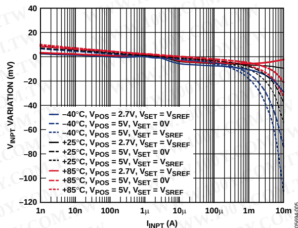
Figure 7. V_{INPT} Variation vs. I_{INPT} for Multiple Temperatures and Voltage, Normalized to V_{POS} = 5\text{ V} , V_{SET} = V_{SREF} , I_{INPT} = 3\text{ }\mu\text{A} and 25^\circ\text{C}
