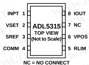
Figure 2. 8-Lead LFCSP
