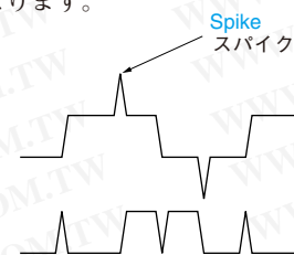
Fig.3 spike waves
