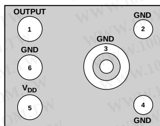
Figure 3. Pin Configuration (Bottom View)
