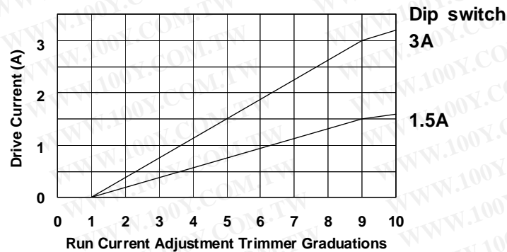
Fig.3. Run Current Setting
