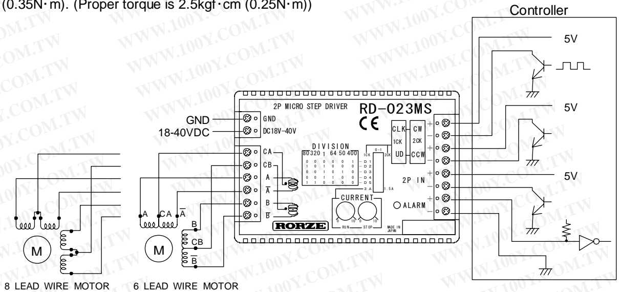
Fig.14. Wiring Diagram
