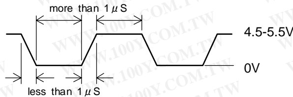
Fig.11. Pulse Specification
