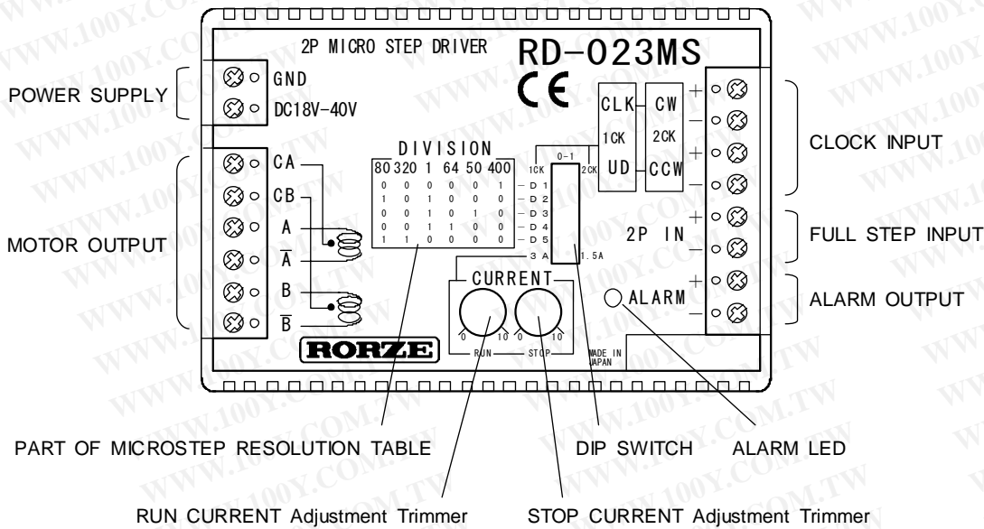
Fig.1. Name Plate
