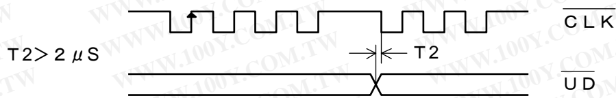
Fig.8. One Clock Timing Diagram
