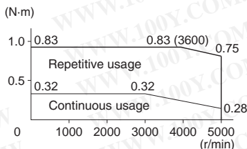
R88M-G10030L/S (100 W)
