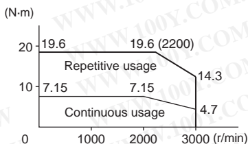
R88M-G1K520T (1.5 kW)
