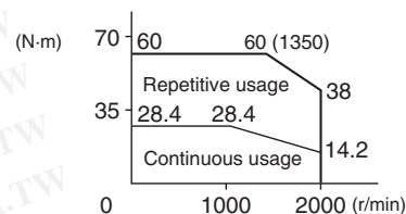
R88M-G3K010T (3 kW)
