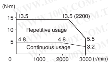
R88M-G1K020T (1 kW)
