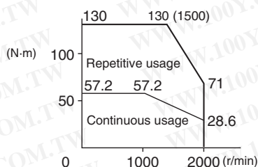
R88M-G6K010T (6 kW)
