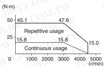
R88M-G4K030T (4 kW)
