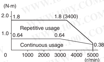
R88M-GP20030L/S (200 W)
