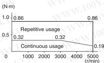
R88M-GP10030H/T (100 W)
