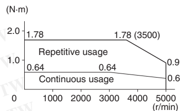
R88M-G20030L/S (200 W)
