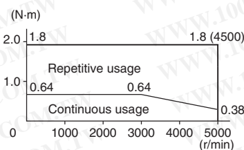
R88M-GP20030H/T (200 W)
