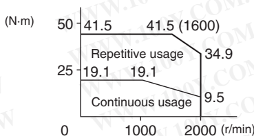
R88M-G6K010T (6 kW)
