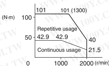
R88M-G4K510 (4.5 kW)
