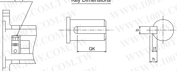
Set bolt (AT)
