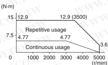
R88M-G1K530T (1.5 kW)
