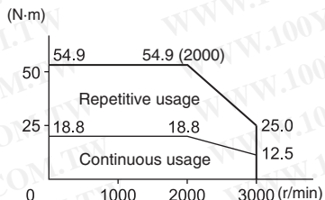
R88M-G4K020T (4 kW)
