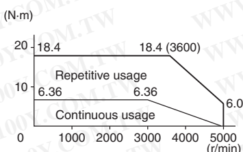
R88M-G2K030T (2 kW)
