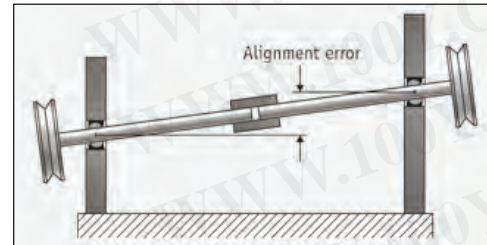
Fig. 9 Shafts located by self-aligning bearings can float into perfect alignment for connection with a solid coupling.
