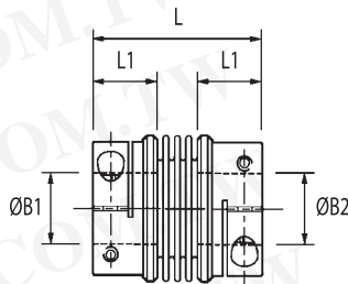
Coupling Type 536 & 537 Short (precisely aligned shafts)
