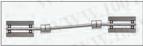
Fig. 7 Two single-stage couplings locate a fully-floating shaft on a stable axis of rotation.
