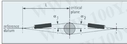
Fig. 2 Maximum radial error = r
