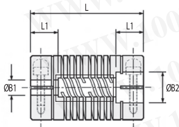
Coupling Type 703 6-Beam Non-Relieved
