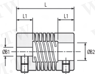
Coupling Type 720 3-Beam Relieved
