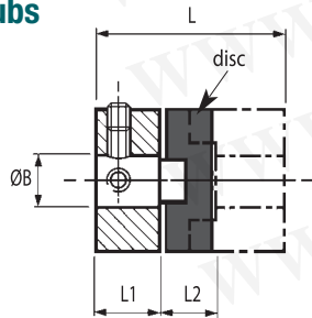
Coupling Type 450 Set Screw style
