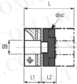
Coupling Type 452 or 453 Clamp style
