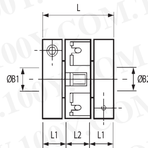
Coupling Type 205 & 206 Integral Leaf Clamp
