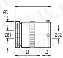
Rigid Coupling Type 281
