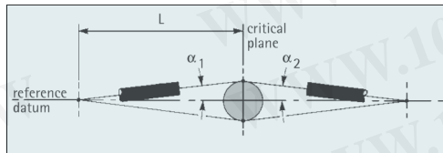
Fig. 3 Maximum parallel error = p_3
