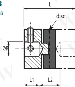
Coupling Type 232 Set Screw style
