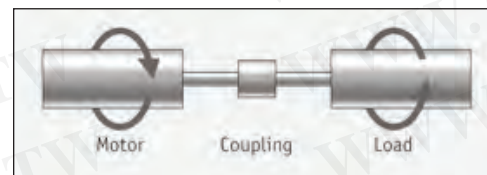
Fig. 10 Mode: Motor accelerates load. Torque 'seen' by coupling = load inertia + frictional resistance of load.
