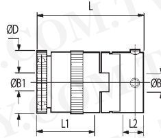
Oldham Coupling Type 285
