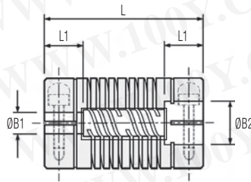
Coupling Type 707 6-Beam Non-Relieved
