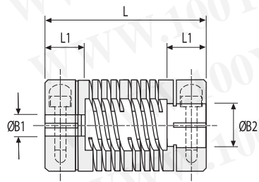
Coupling Type 727 6-Beam Relieved
