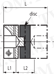
Coupling Type 234 & 235 Clamp style
