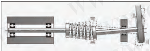
Fig. 8 A semi-floating shaft located by a self-aligning bearing at one end and a multi-stage bellows at the other. The coupling reacts to fluctuating tension in the belt by allowing lateral oscillations in the shaft.
