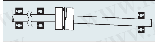
Example 1. With partially supported (1 bearing) shafts.
