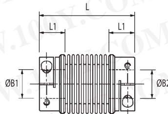
Coupling Type 555 Long (greater angular offsets or axial motion)
