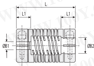
Coupling Type 723 6-Beam Relieved
