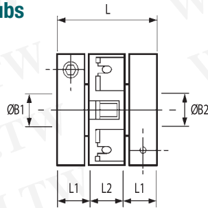
Coupling Type 207 Collet Hub and Ring Clamp
