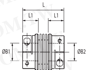
Coupling Type 554 Short (precisely aligned shafts)
