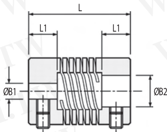
Coupling Type 724 3-Beam Relieved
