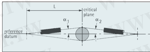
Fig. 4 Worst case radial error r_2 = p_3 + r
