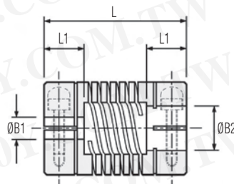
Coupling Type 721 3-Beam Relieved
