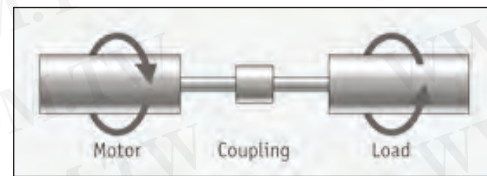
Fig. 11 Mode: Supply to motor discontinued, braking applied to load. Torque 'seen' by coupling = motor inertia - motor drag.
