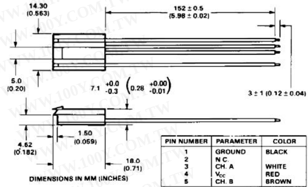
Figure 6. HEDS-8902 Connector.
