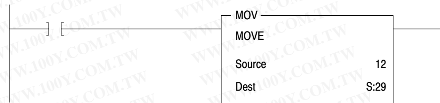
Figure 7.5 Example of Changing the Fault Routine File Number
