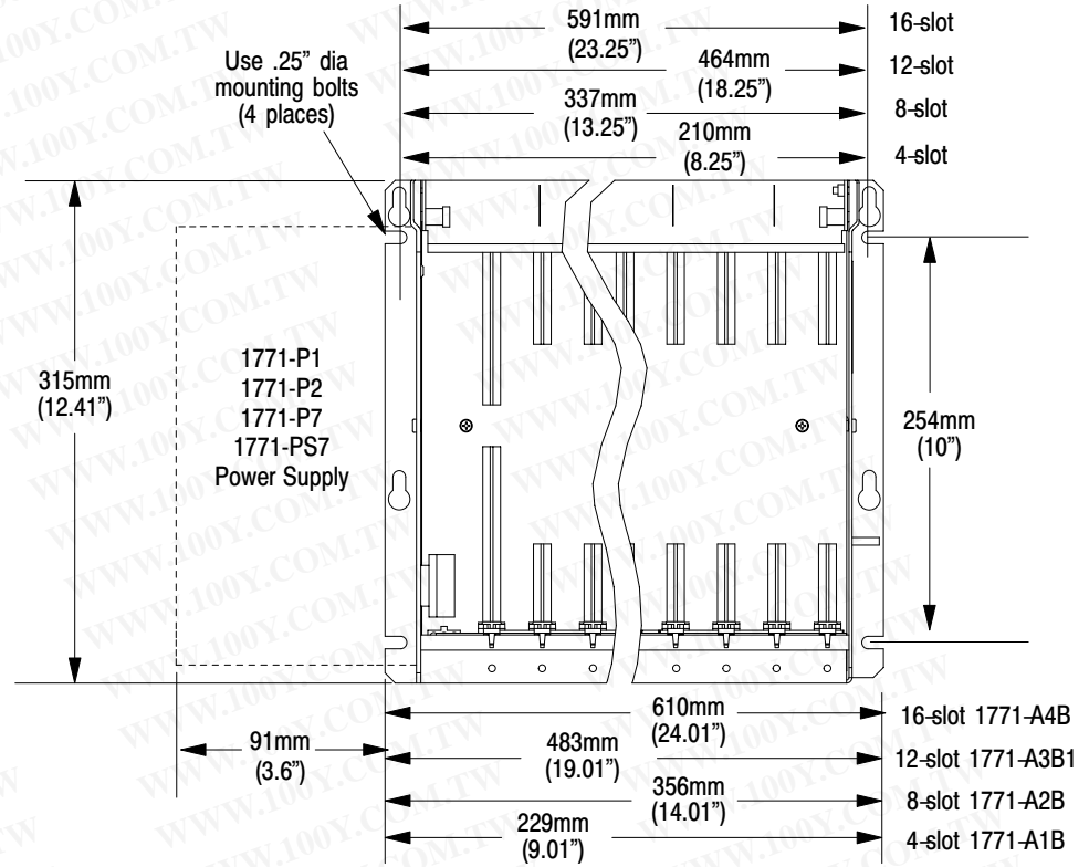
Figure 3.2 I/O Chassis and 1771-P2 Power Supply Dimensions
