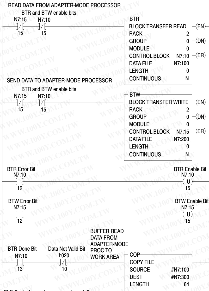
Figure 8.8 Example Block Transfer in PLC-5 Supervisory Processor
