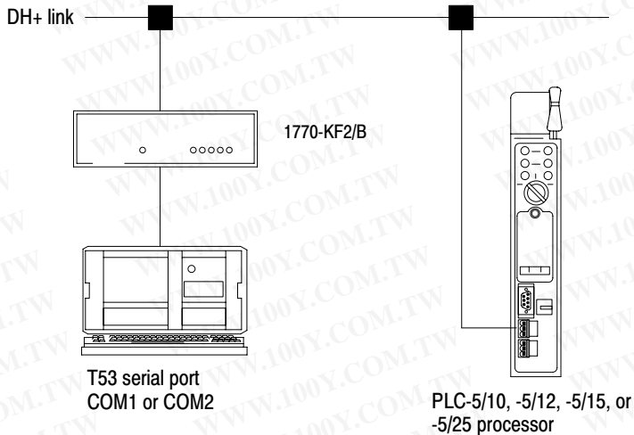
Figure 5.12 1770-KF2/B Connection through an RS-232-C Serial Port
