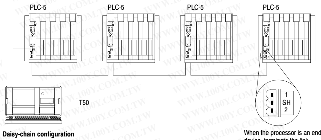
Figure 5.7 Examples of DH+ Link Connections (Daisy-Chain and Trunkline/Dropline)
