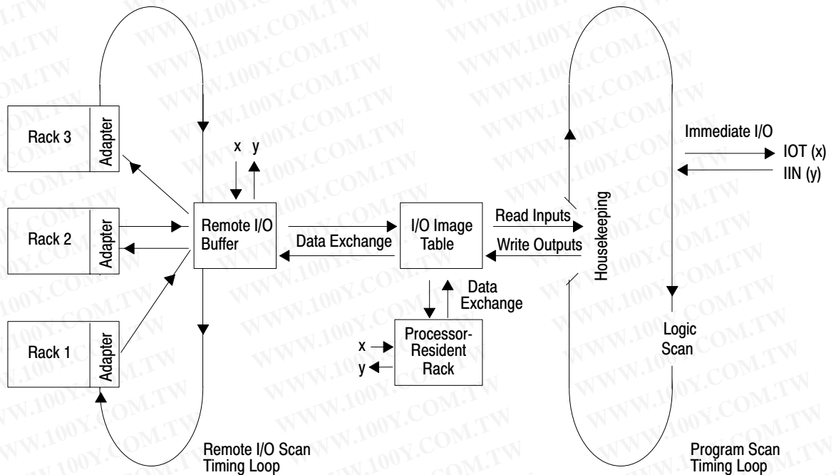
Figure 9.1 Remote I/O Scan and Program Scan Timing Loops
