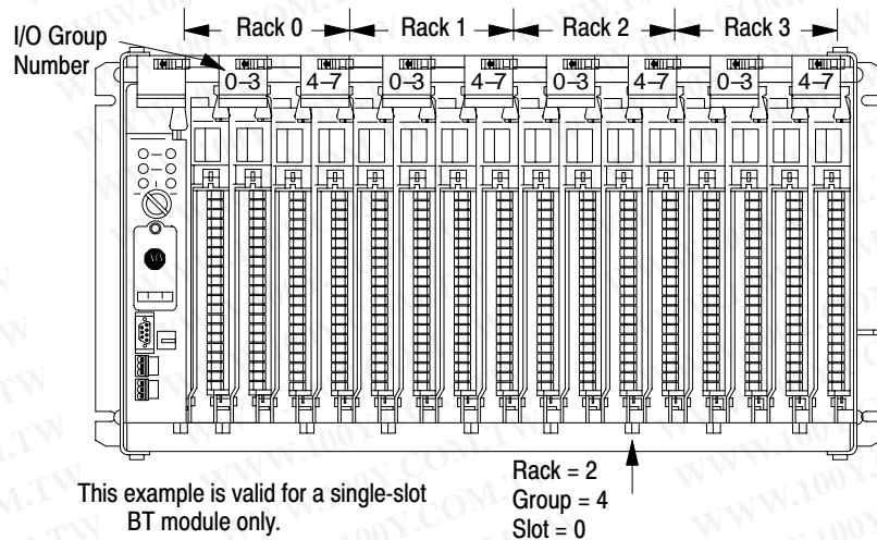
Figure 4.4 Example Block-Transfer Module Address Using 1/2-Slot Addressing
