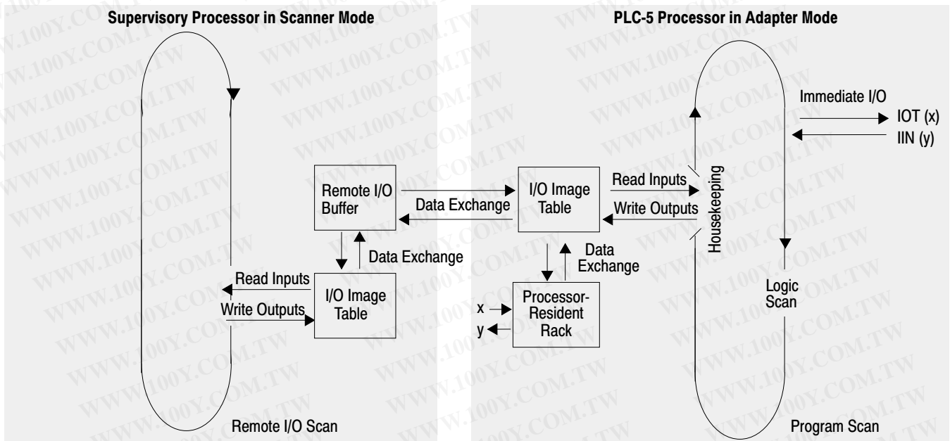
Figure 8.1 shows the transfers between supervisory processor output file and adapter-mode processor input file as well as between adapter-mode processor output file and supervisory processor input file.
