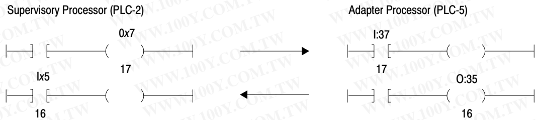
Figure 8.2 Transferring Bits Using Rack 3 in the Adapter-Mode Processor
