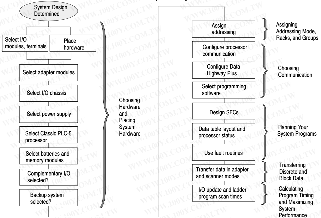
Figure 1.1 PLC-5 Processor System Design Flow
