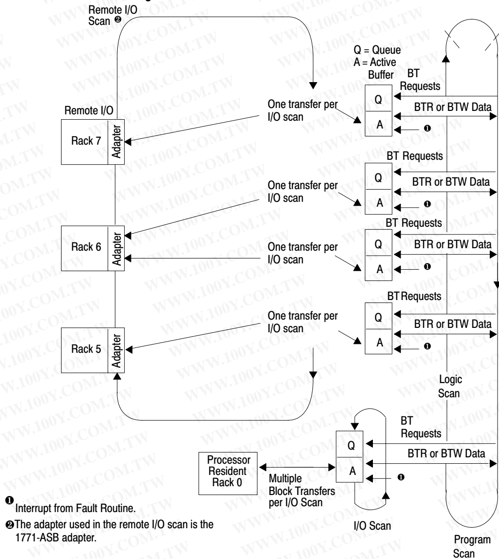
Figure 9.2 Transferring Block Data to Local and Remote I/O
