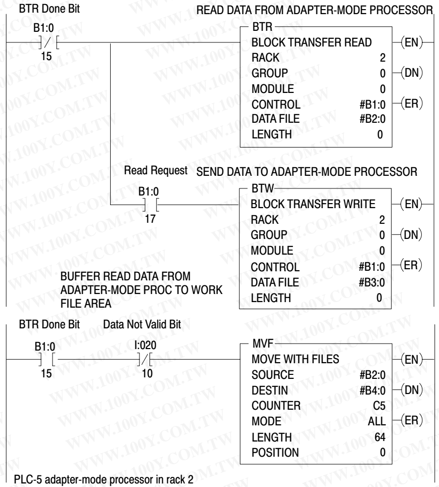
Figure 8.7 Example Block Transfer in PLC-3 Supervisory Processor
