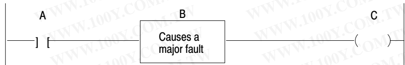
Figure 7.3 Sample Ladder Logic for a Fault
