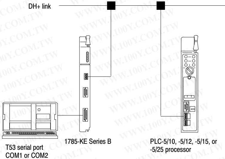
Figure 5.11 1785-KE (Series B) Connection through an RS-232-C Serial Port
