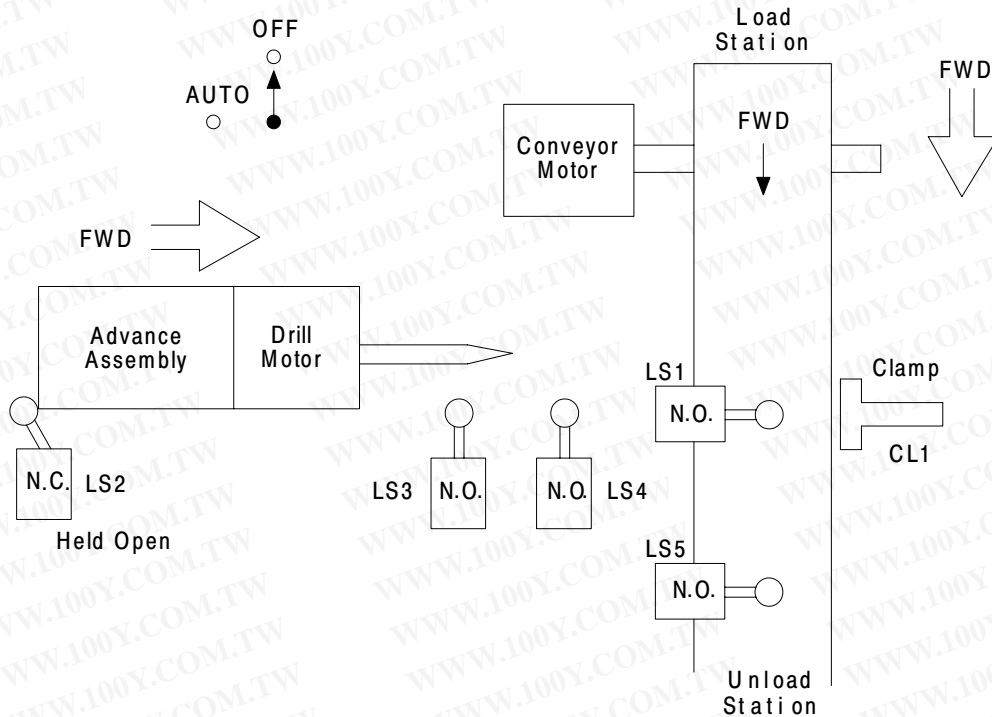
Figure 6.1 Hardware Block Diagram and Description of Machine Process
