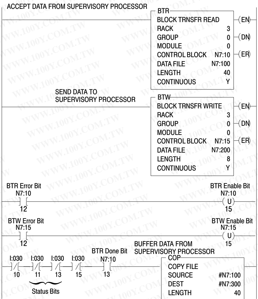
Figure 8.10 Example Block Transfer for a PLC-5/12, -5/15, or -5/25 Processor in Adapter Mode
