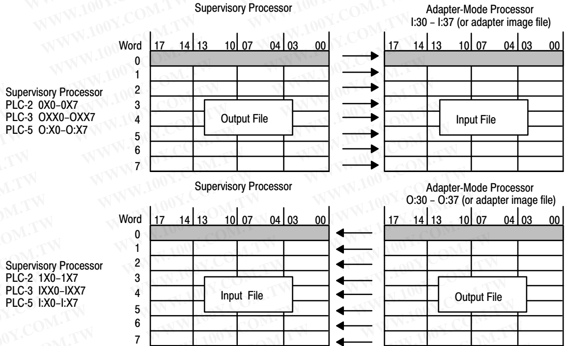
Figure 8.1 Automatic I/O Transfer between Supervisory and Adapter-Mode Processors
