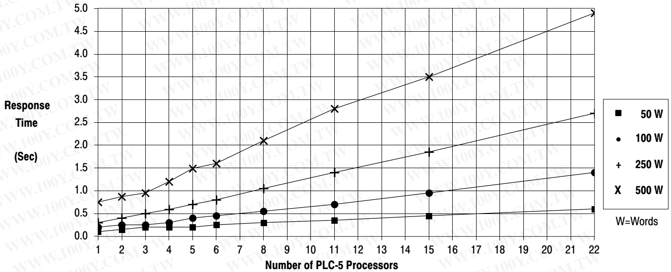
Figure 5.5 Average Response Time for all PLC-5 Processors
