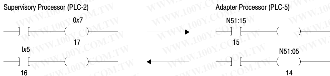
Figure 8.3 Transferring Bits Using Your Own Adapter Image File
