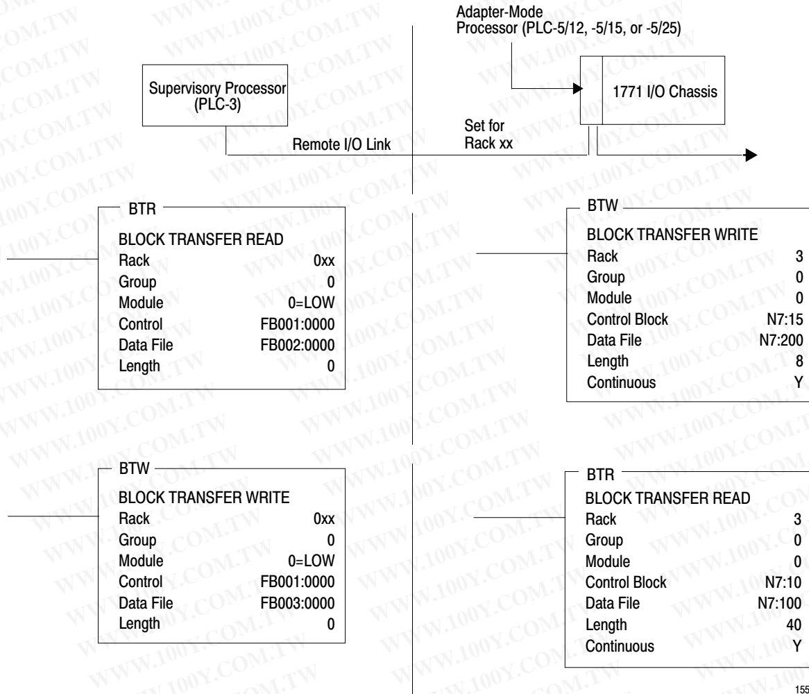
Figure 8.4 Example Adapter/Supervisor Block-Transfer Programming for a PLC-5/12, -5/15, or -5/25 Adapter-Mode Processor in Rack xx
