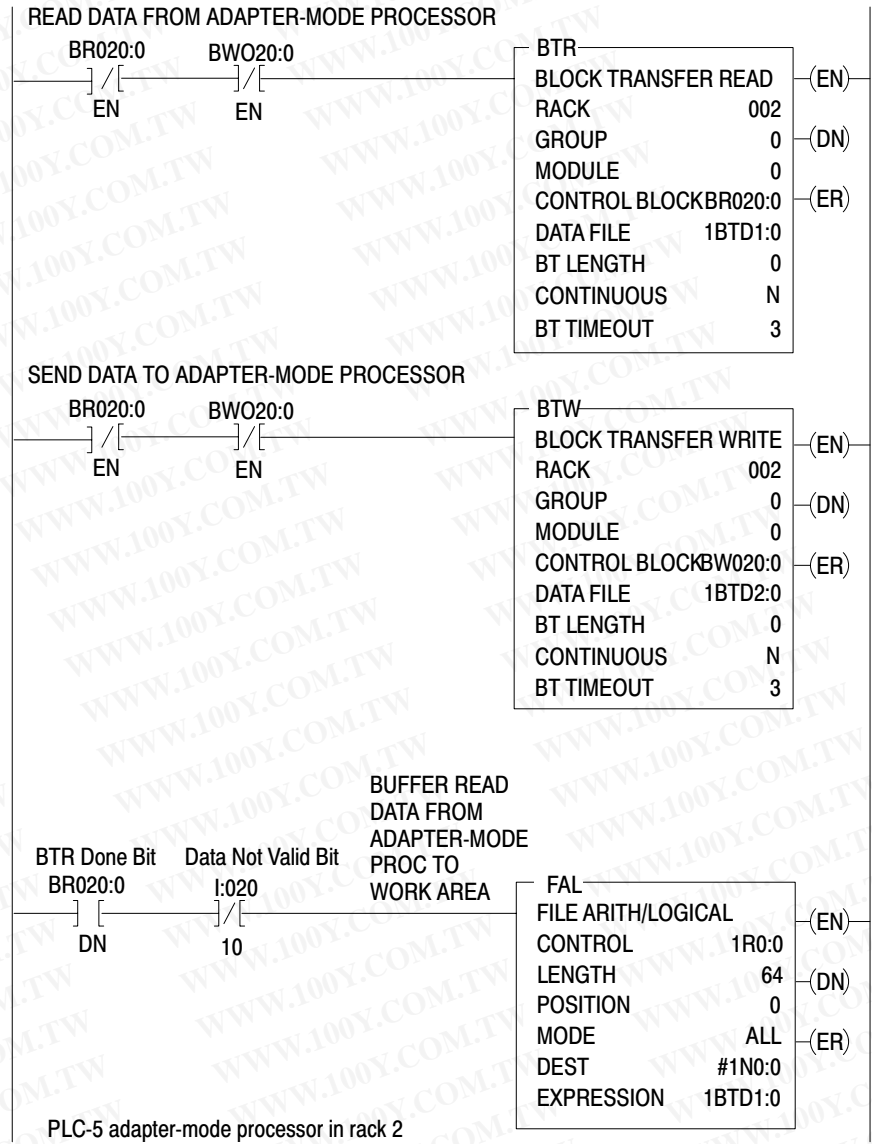
Figure 8.9 Example Block Transfer in PLC-5/250 Supervisory Processor
