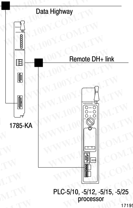
Figure 5.10 Example DH+ to Data Highway to DH+ Link Configuration
