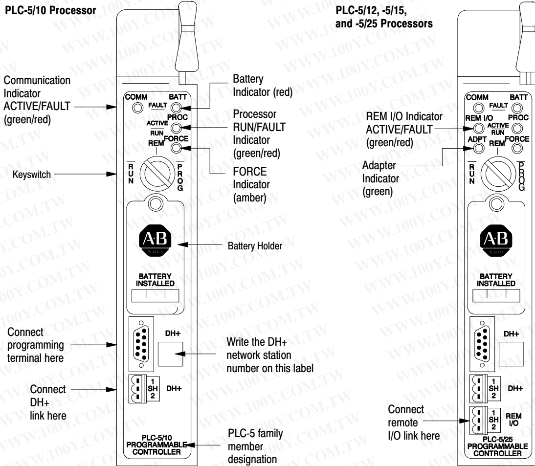
Figure 5.1 Processor Front Panels
