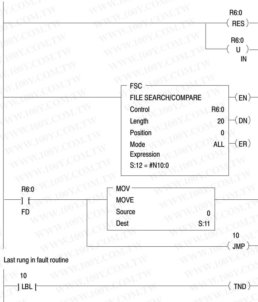
Figure 7.4 Example of Comparing a Major Fault Code with a Reference
