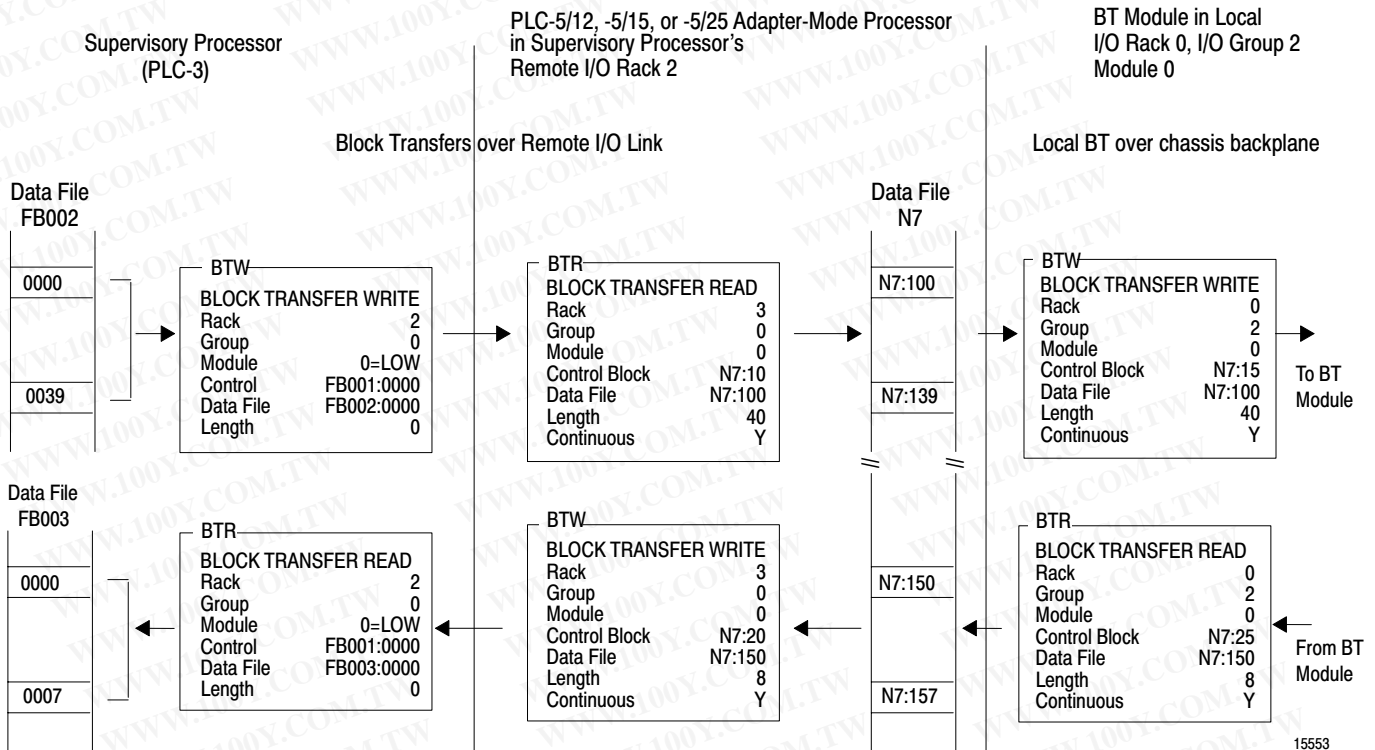
Figure 8.5 Example Block Transfer from Supervisory Processor to a PLC-5/12, -5/15, or -5/25 Adapter-Mode Processor to Local Block-Transfer Module and Vice Versa
