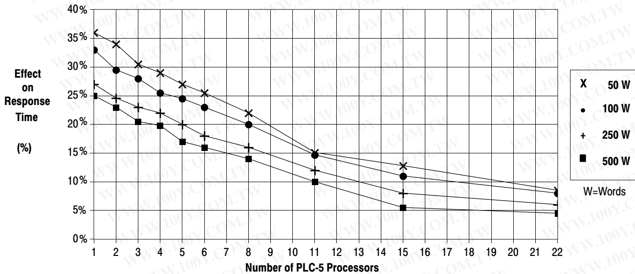
Figure 5.6 Response Time Increase (%)
