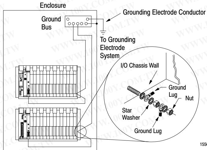
Figure 3.3 Recommended Grounding Configuration for Remote I/O Systems
