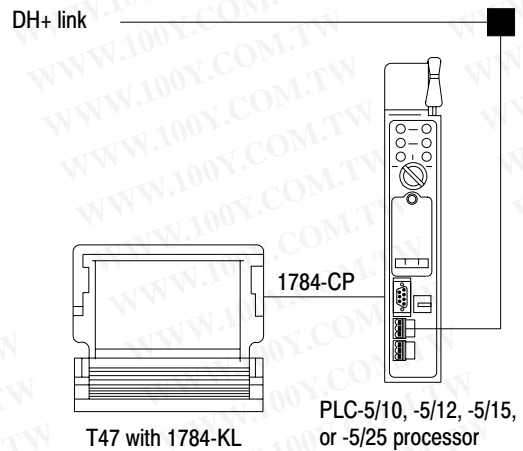
Figure 5.9 Connection to DH+ Link through 1784-KL Communication Interface Module
