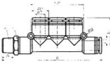
● YPKB/TPKB 螺纹五通
