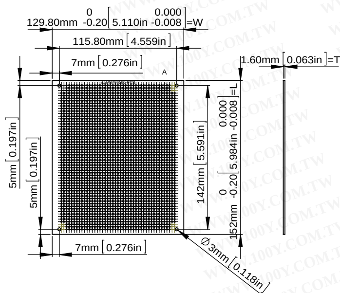
ALUG706160-PCB
