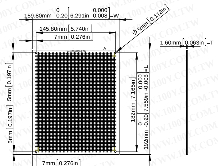
ALUG708200-PCB
