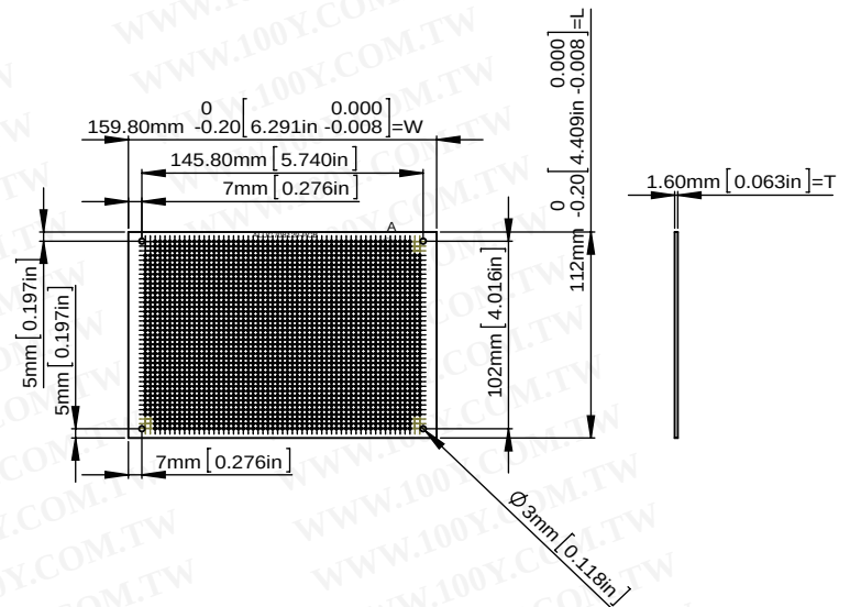
ALUG708200-PCB
