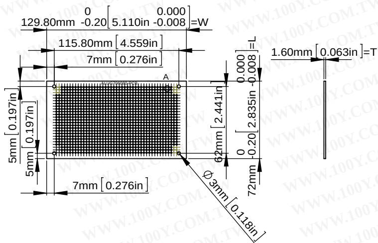
ALUG706160-PCB
