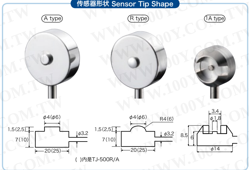
传感器形状 Sensor Tip Shape
