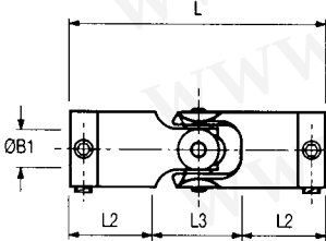
Ref. 103 Headed brass inserts fitted 2 screws per end (size 6, one screw)
