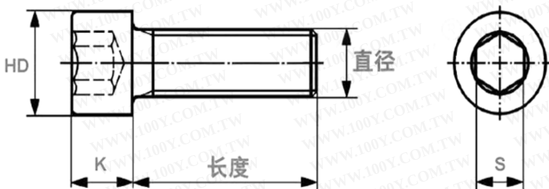
DIN912 Hex Socket Head Cap Screw
