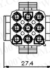
9, 12, 15 Circuit (Matrix)
