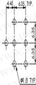
2, 3, 4 Circuit (In-Line)
