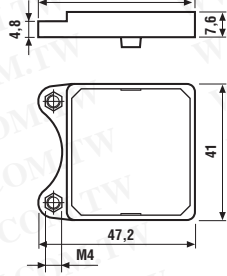
Mounting adaptor for types 62.3x and 62.8x.xxxx.xxx9 (M4)
