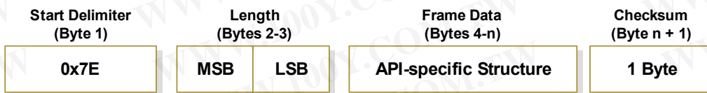
Figure 3-01. UART Data Frame Structure:
