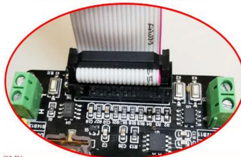
JTAG Debug interface for 20Pin 2.54MM
