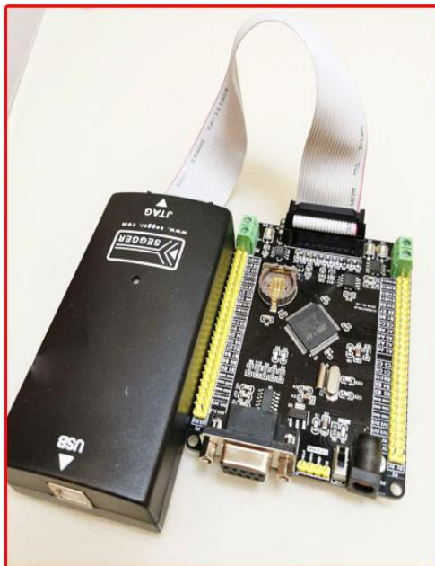
JTAG Debug interface for 20Pin 2.54MM
