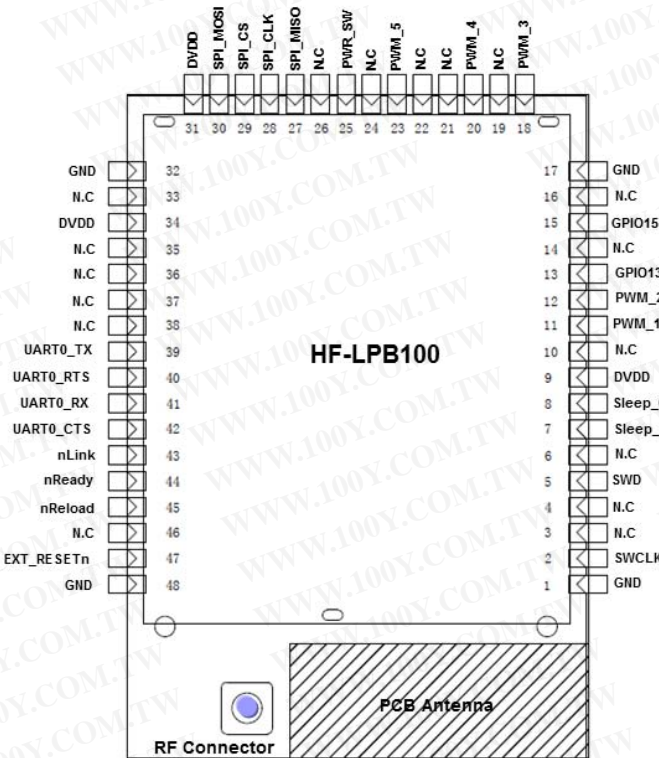
Figure 2. HF-LPB100 管脚定义
