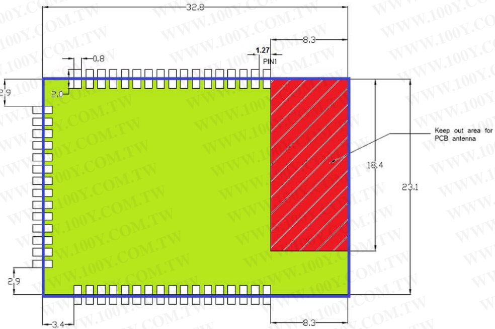
Figure 4. HF-LPB100 PCB 元件尺寸
