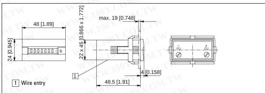
Panel cut-out
