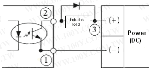
(Transistor Output)
