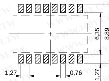
Land Pattern
