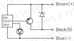
3 wire PNP solid state circuit
