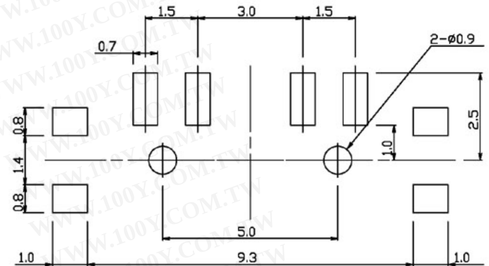
P.C.B MOUNTING HOLES
