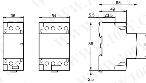
iCT 40/63 A
