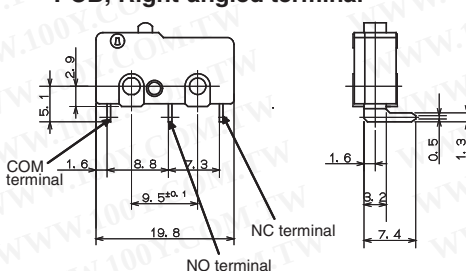
PCB, Right-angled terminal
