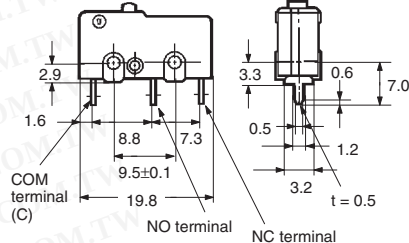
PCB Terminals
