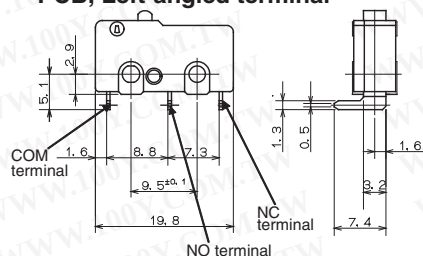
PCB, Left-angled terminal
