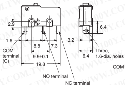
Solder Terminals
